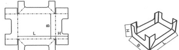
FEFCO 0770
