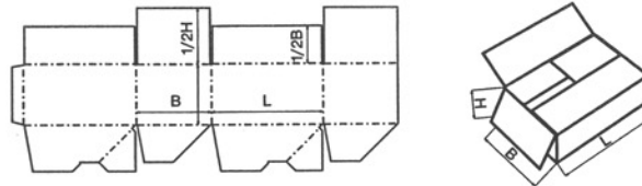
FEFCO 0713
