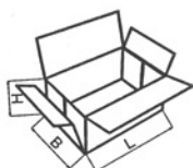
FEFCO 0416
