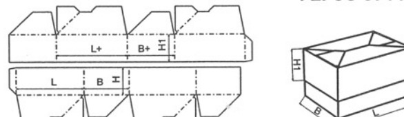
FEFCO 0714
