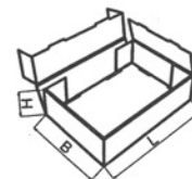
FEFCO 0426
